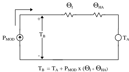
Figure 10a Thermal model for convection cooled systems.
