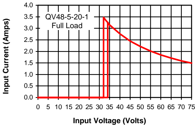
Input Characteristics
