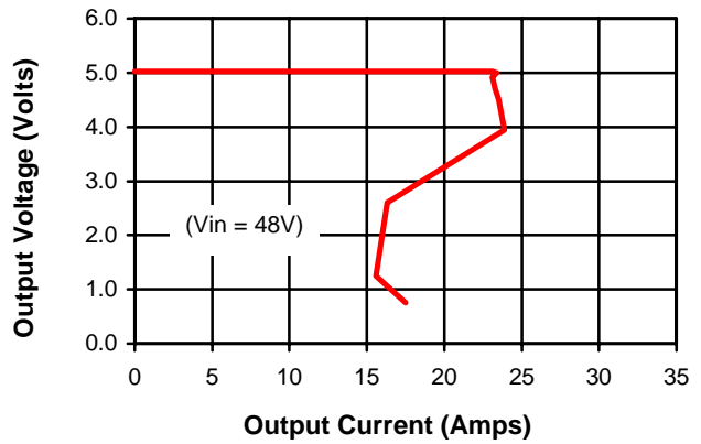
Output Characteristics
