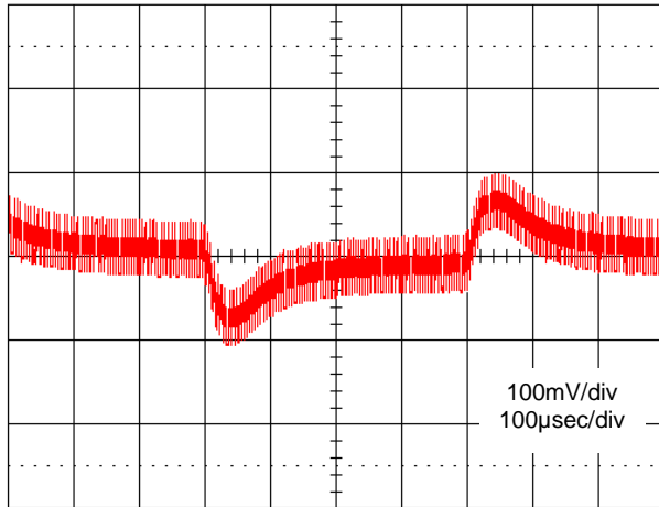
Transient Response
